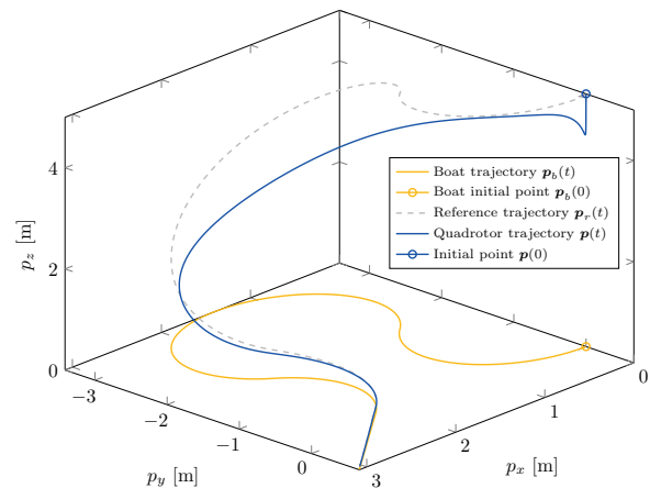
Fig. 5. Perspective view of the landing scenario
